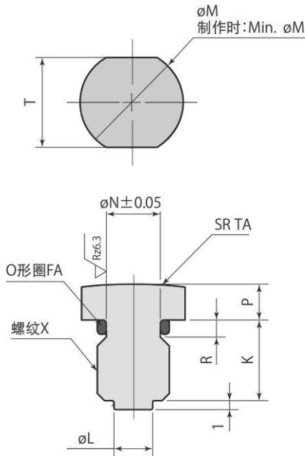
帽盖详图硬度HRC52
