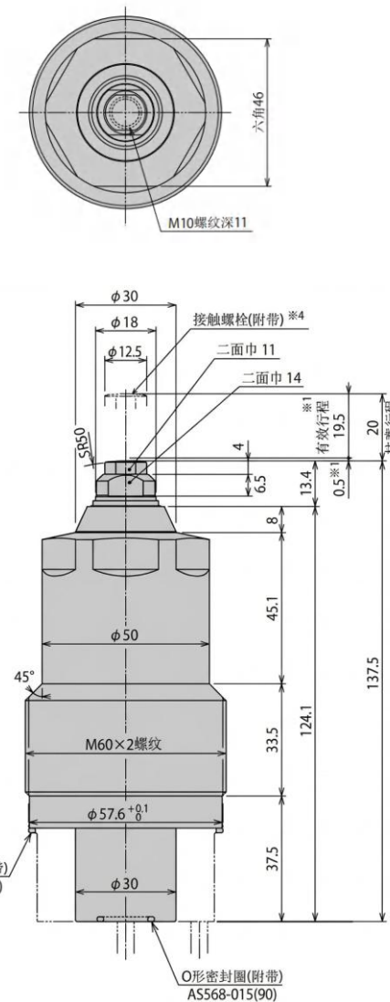
帽盖详图 HRC52
