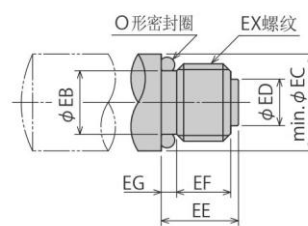
帽盖详图硬度HRC52
