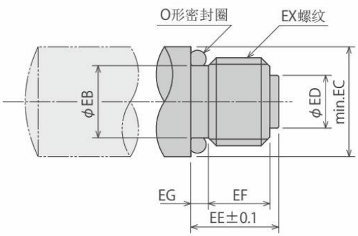
帽盖详图硬度HRC52
